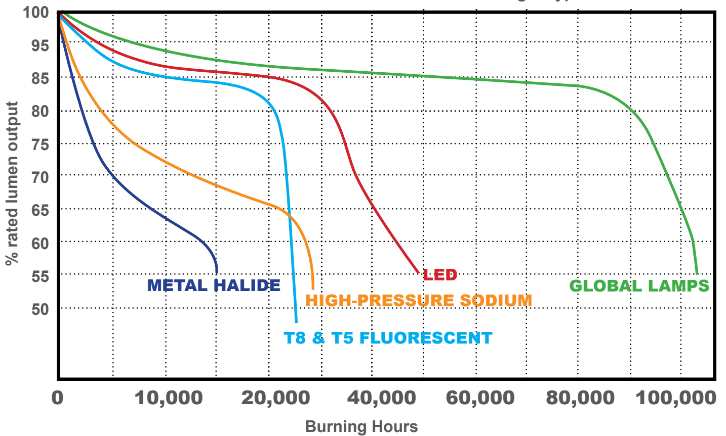
Lumen Maintenance Curves For Various Commercial Light Types
